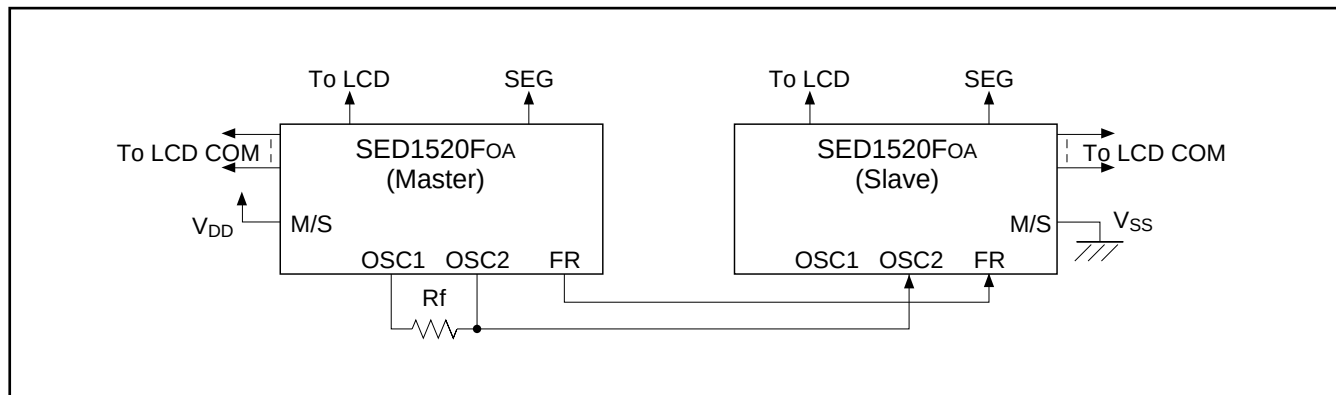
Figure 7.1. SED1520FOA – SED1520FOA
