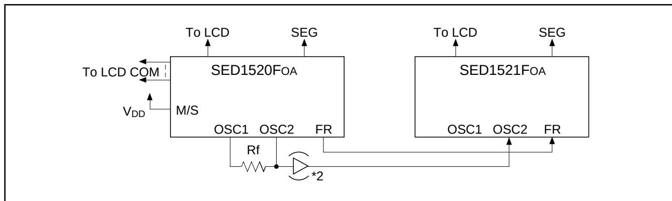
Figure 7.3 SED1520FOA – SED1521FOA *1
