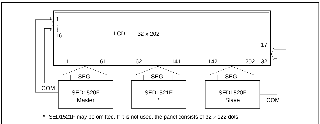
Figure 8.3. Duty 1/32, 33 characters \times 4 lines
