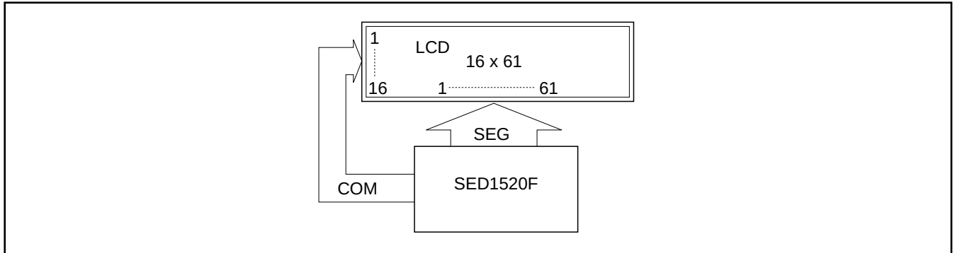
Figure 8.1. Duty 1/16, 10 characters \times 2 lines
