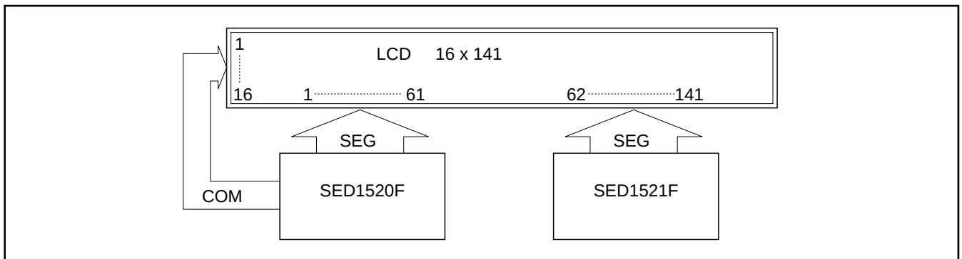
Figure 8.2. Duty 1/16, 23 characters \times 2 lines
