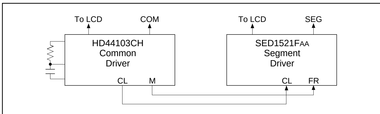
Figure 7.5. HD44103CH – SED1521FAA
